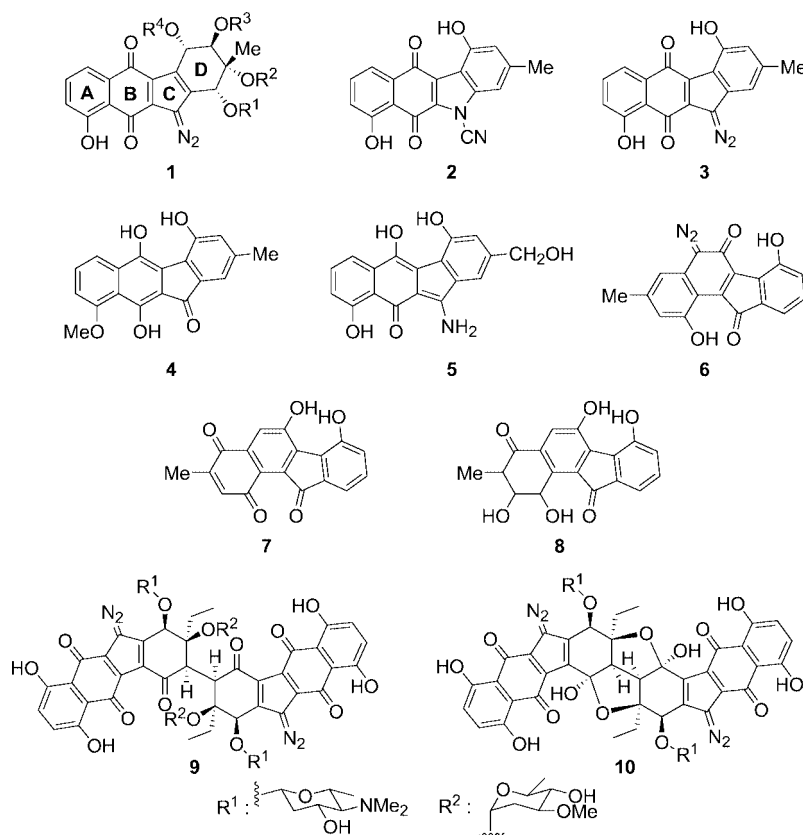
Figure 1. Kinamycins and related naturally occurring compounds.
